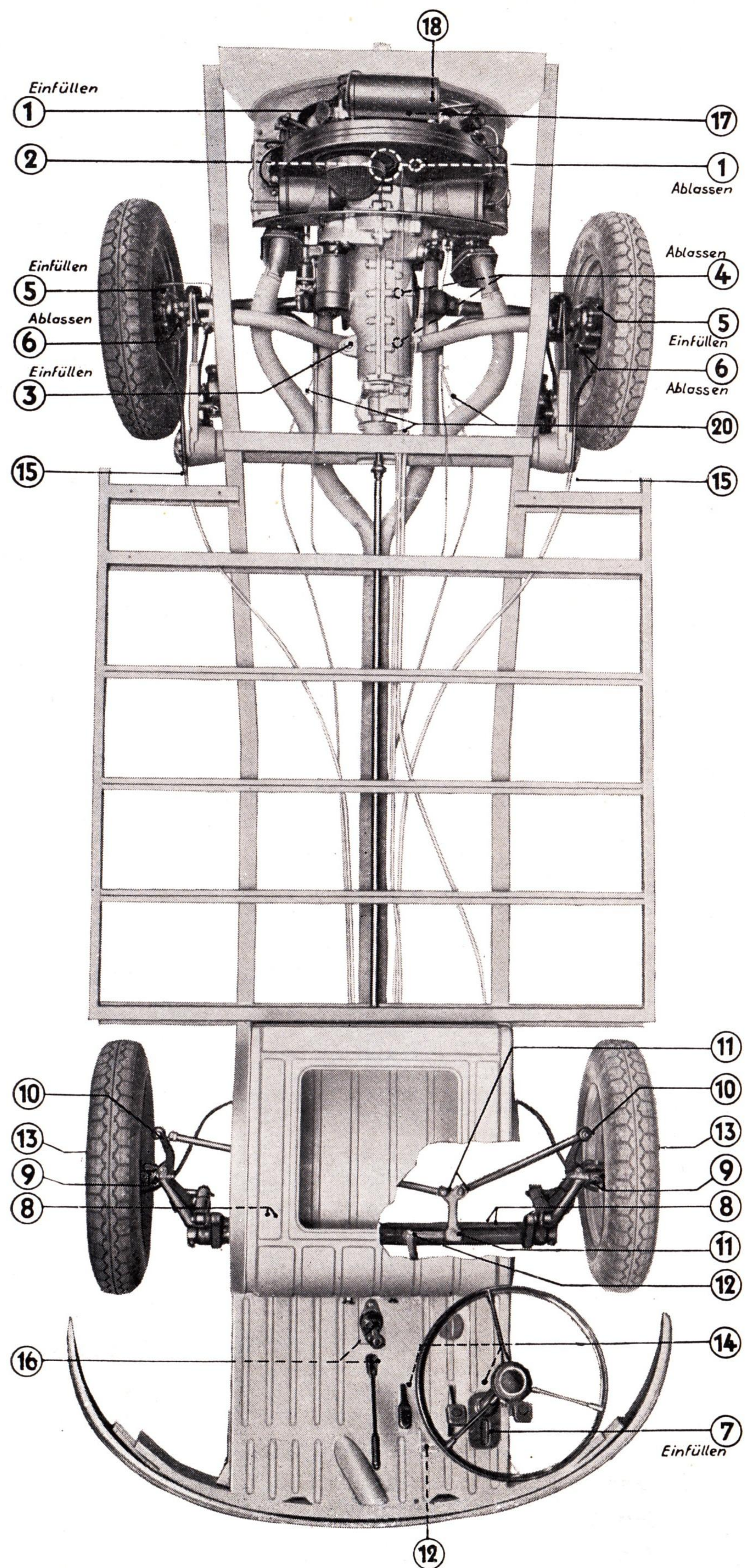
VW-Transporter
