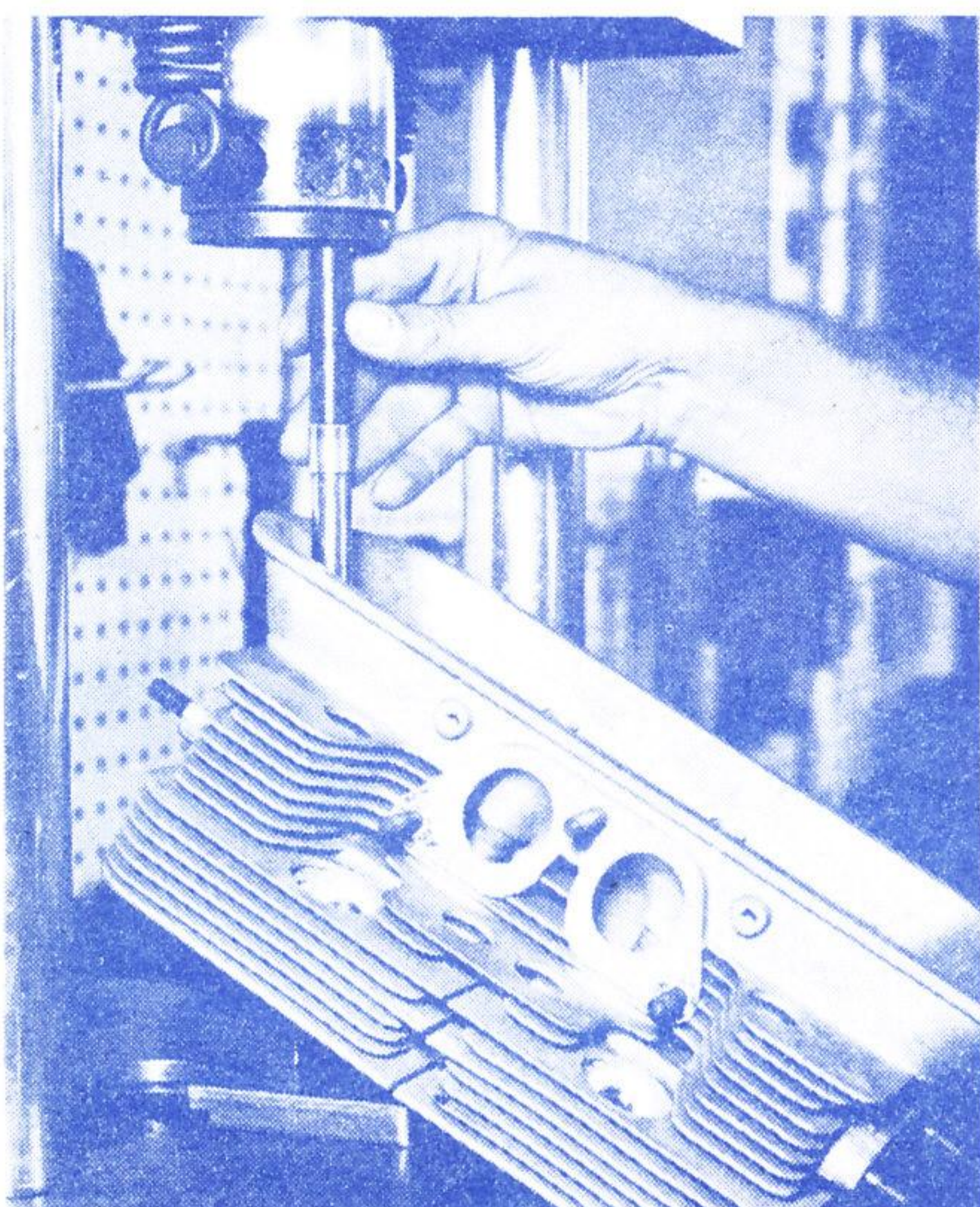
INSTALLING PORSCHE EXHAUST GUIDE
