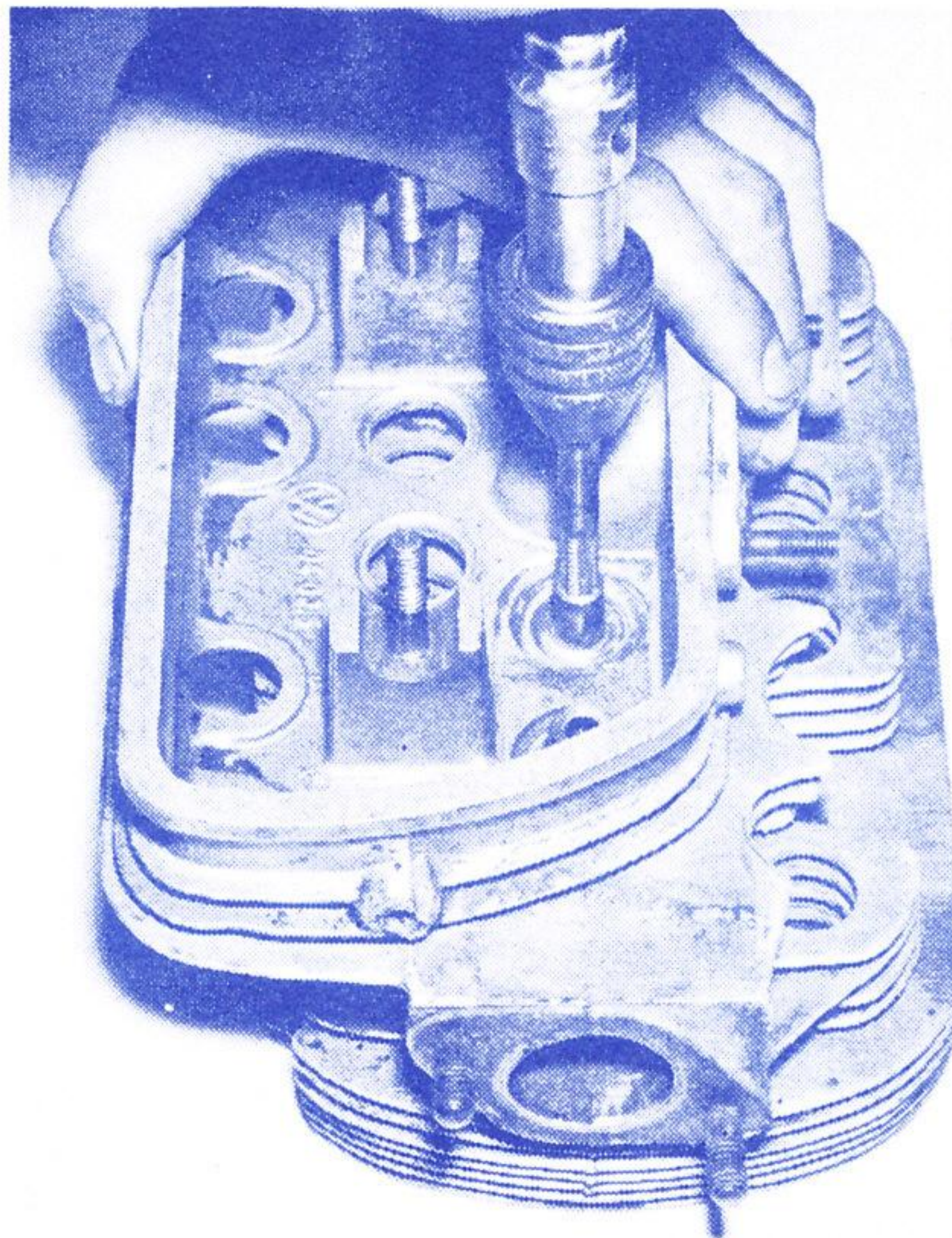
TAPPING WORN GUIDE VW HEAD
