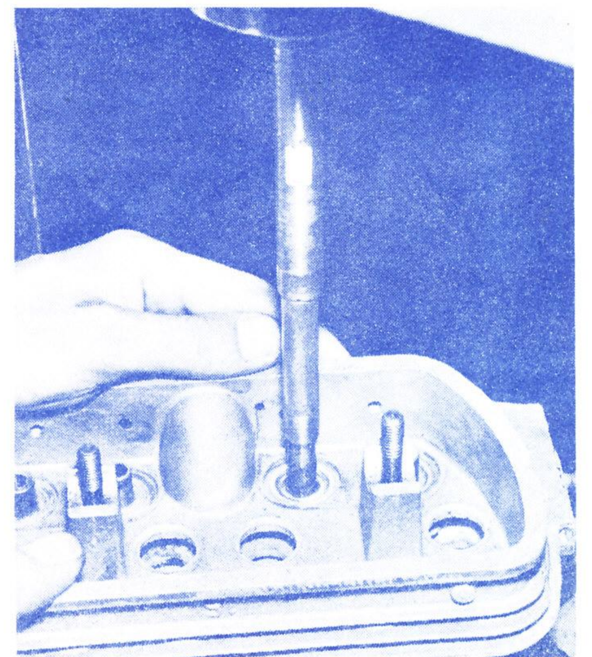
GUIDE ALMOST SEATED VW HEAD
