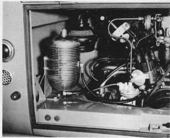
E.M.P.I. Filter Cooler installation on VW Transporter.
